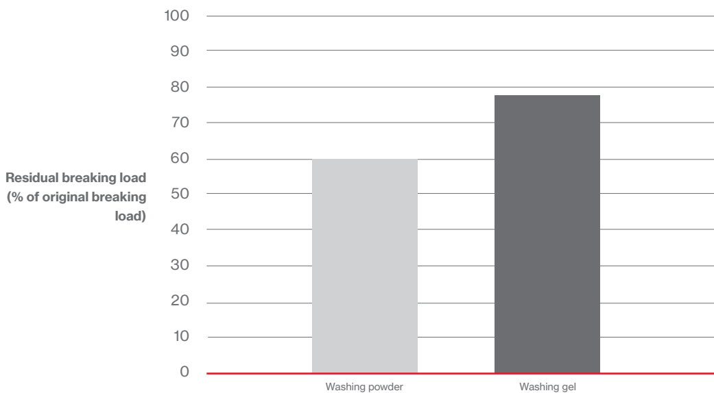
Comparison of detergents - loss of breaking load of a polyester rope
