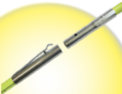
Aluminum heavy duty ferrules with external leaf spring locking button
